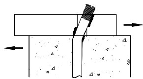
Mode III - wood bearing deformation in side member & dowel bending in concrete.
