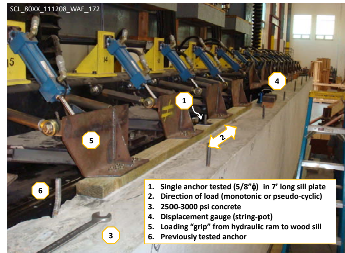
Image 1 – Annotated view of the typical testing set-up.
