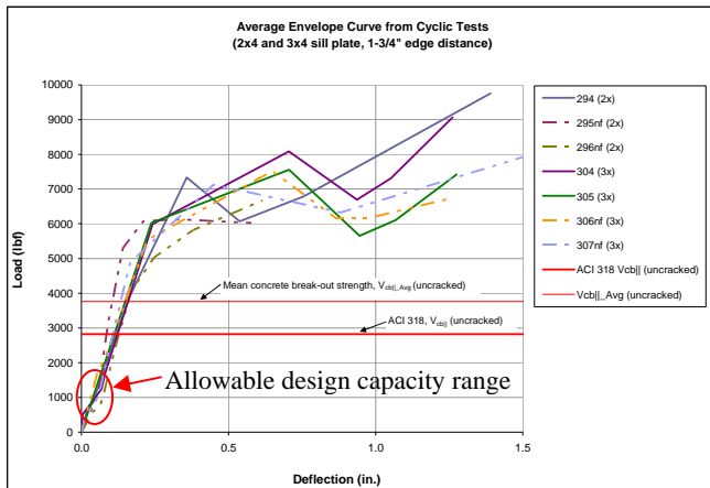
Chart 1 – Envelope curve (Chart 9 in full report)
