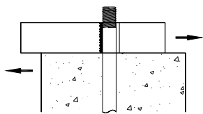
Mode I - wood bearing deformation in side member.
